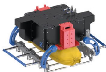
Hold-down device
